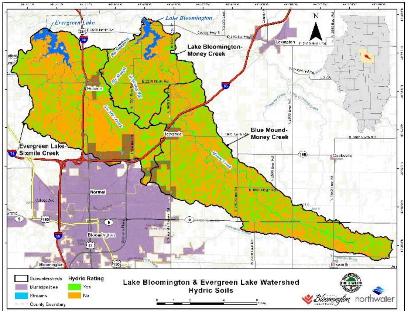
Figure 24 – Hydric Soils
