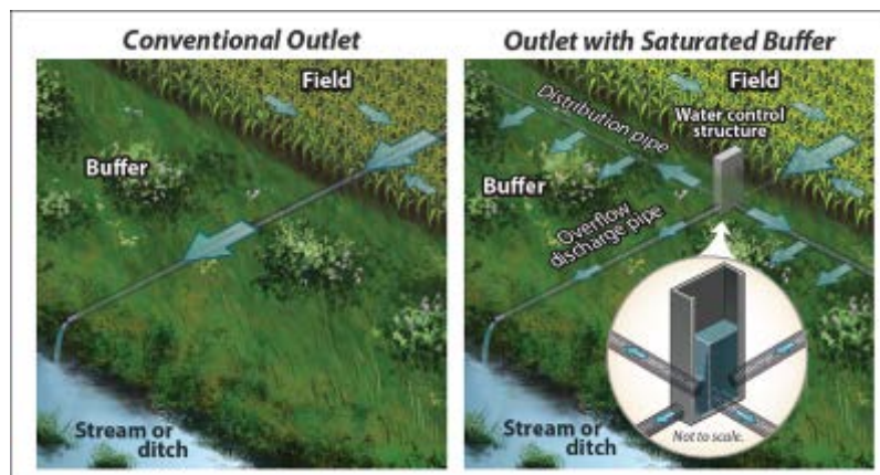
Saturated Buffer - Credit: USDA
