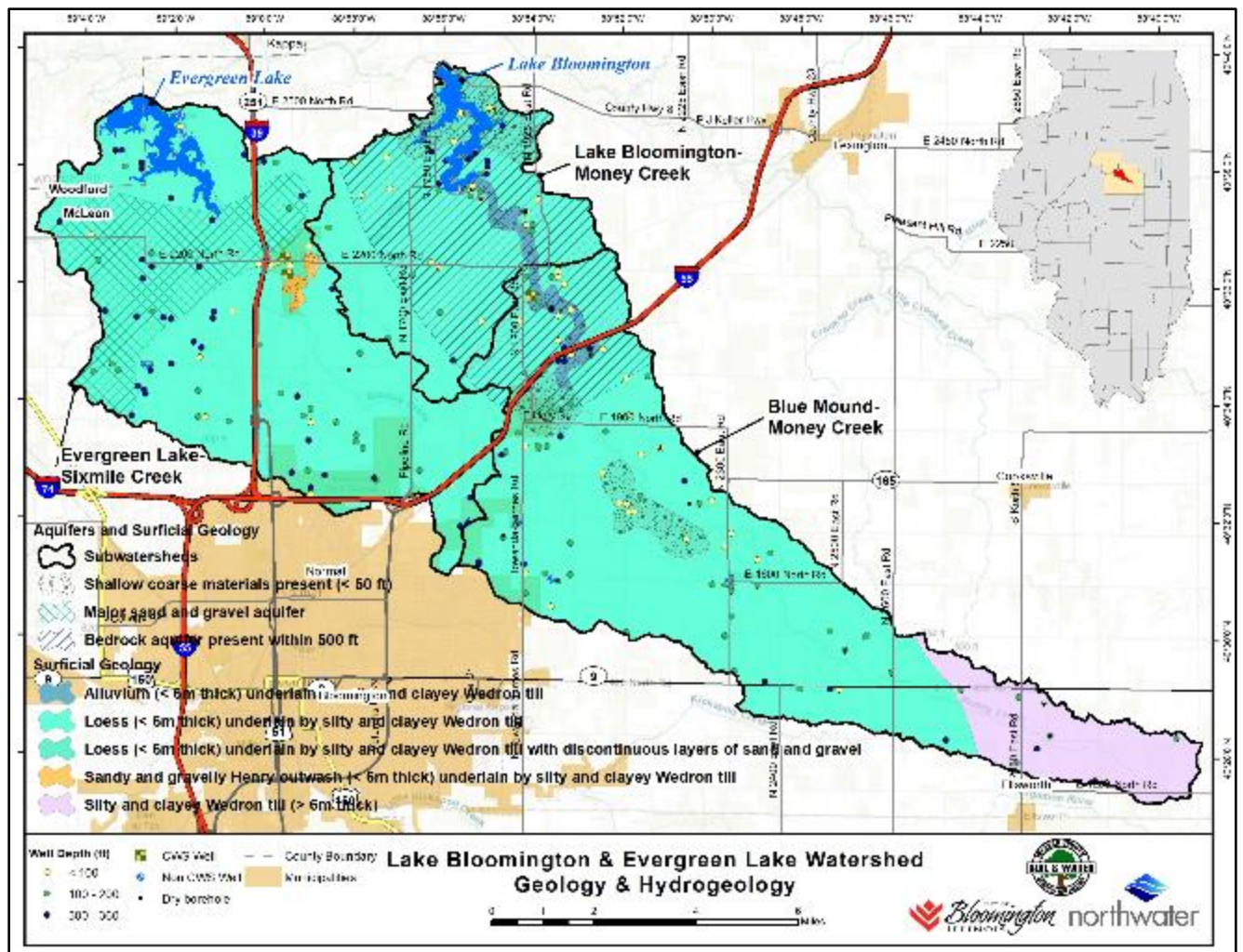
Figure 18 – Geology & Wells
