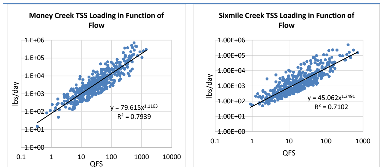
Figure 15 - Relationship Between TSS Loading & Flow
