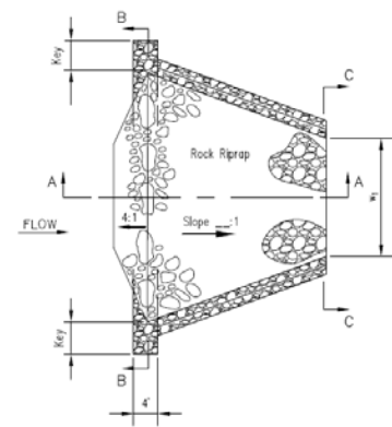
NRCS Riffle Detail
